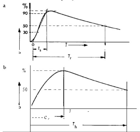
Fig. 4 Standardized test voltages a Lightning impulse voltage 1.2/50 Front time: T_f = 1.2 \pm 0.36 \mu\text{s} Time of half value: T_r = 50 \pm 10 \mu\text{s} b Switching impulse voltage 250/2500 Front time: T_{fr} = 250 \pm 50 \mu\text{s} Time of half value: T_h = 2500 \pm 1500 \mu\text{s}
